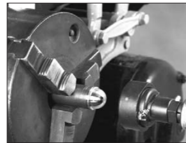
Lathe with Large Extended Series.
